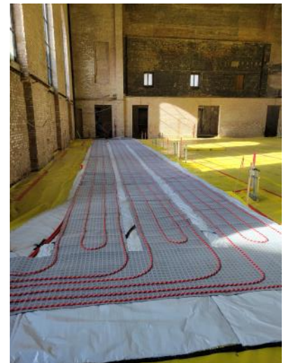
Radiant heat tubing ready for concrete floor
